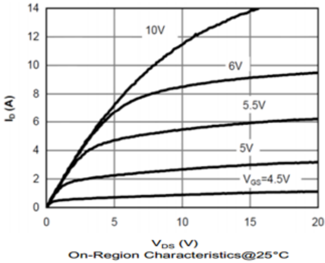
Output Characteristic
