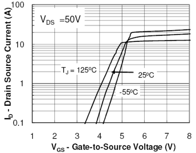
Transfer Characteristic
