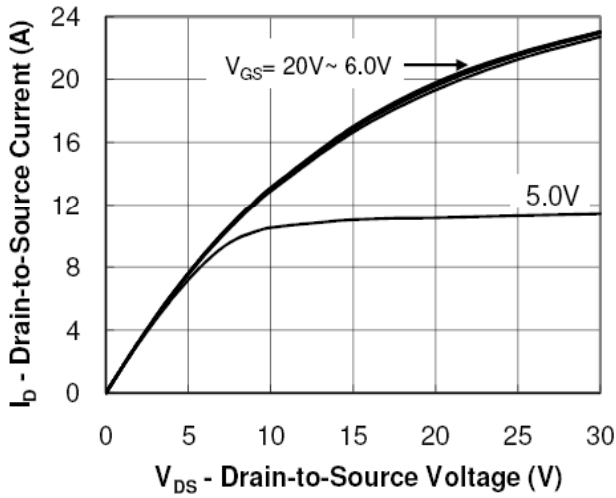
Output Characteristic
